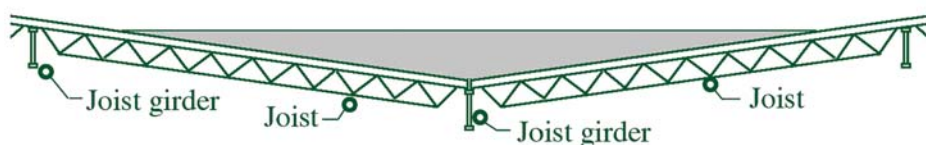
(b) Joists parallel to roof slope, meeting in a valley
