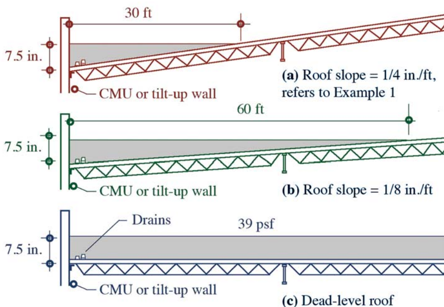
Figure 11 – Effect of roof slope on rain load on a roof. The maximum rain load in all three illustrations is 39.0 psf. The rain load distribution shown in illustration (a) relates to the building of Example 1.
